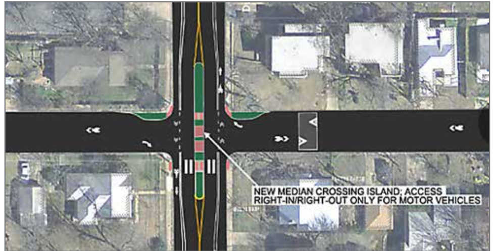
Proposed Median Crossing at Duval and 47th Street
